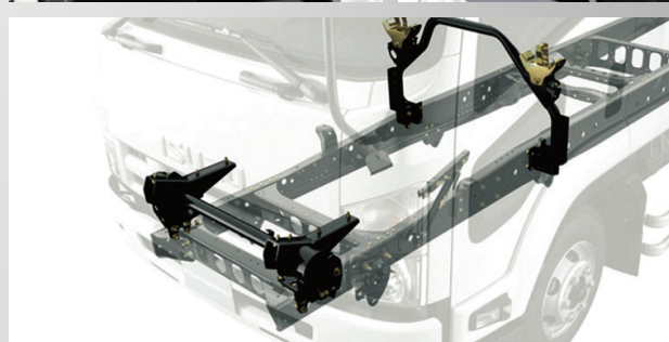
▲ Full floating cabin.
