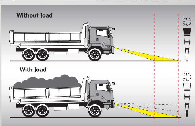
▲ Headlight leveling. Preferred headlight beam position can be maintained when truck is loaded and when it has no load.
